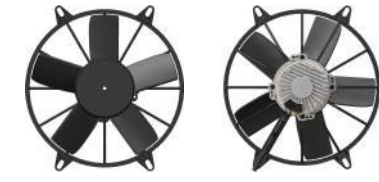
11" (280mm) STRAIGHT BLADE
