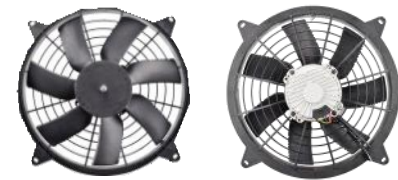
12" (305mm) S-BLADE
