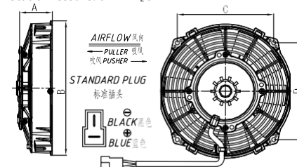
CONNECTOR(插头), AMP 180908 TERMINAL(插片), AMP 42098-2
