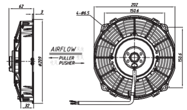
7.5" (190mm) ECONOMICAL REVERSIBLE STRAIGHT BLADE
