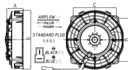
CONNECTOR(插头), AMP 180908 TERMINAL(插片), AMP 42098-2
