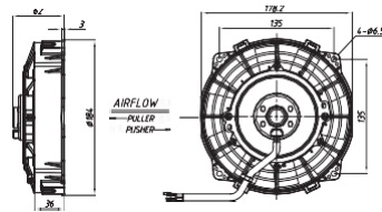
7.5" (190mm) ECONOMICAL REVERSIBLE STRAIGHT BLADE
